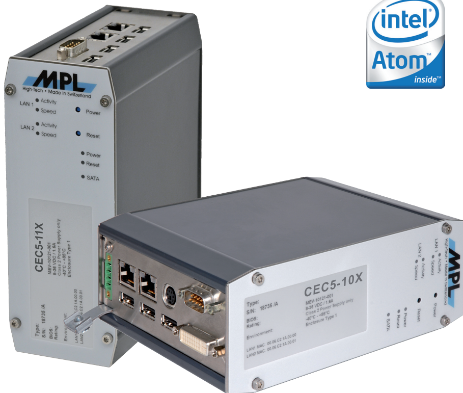
CEC5-X dimensions: 62 x 162 x 120 mm (W x H x D) Compact rugged aluminum housing with stainless steel side plates
