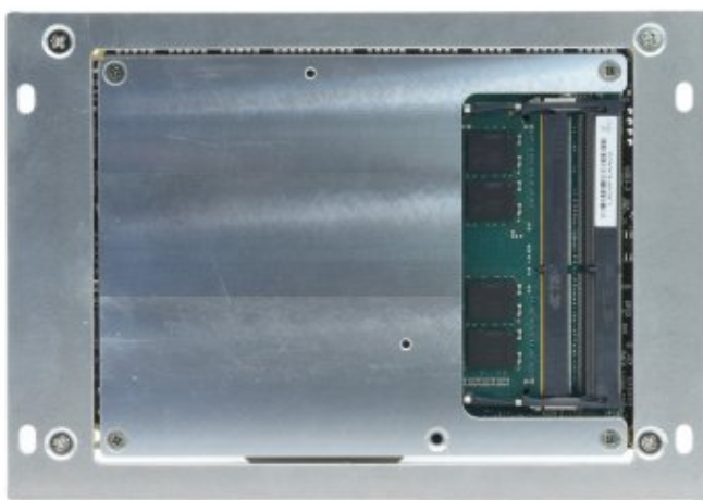
Jasper SBC bottom view showing mounting plate (outer) and COM heat spreader (inner)
